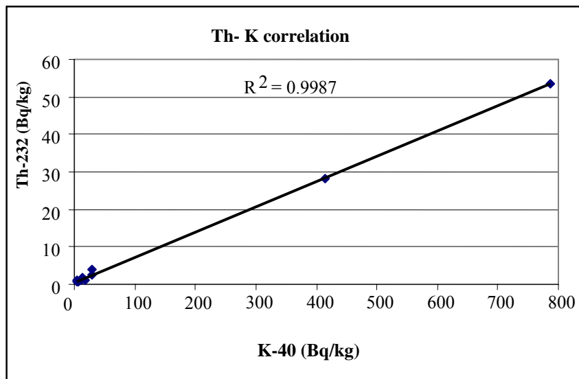
Fig.5. Correlation between 40 K and 232 Th.
