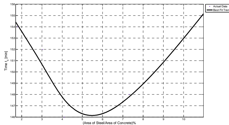
Figure 12: Effect of Reinforcing Ratio on the Time of Failure
