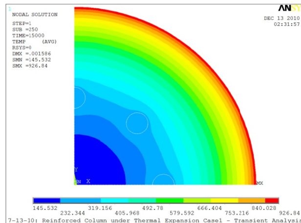
Figure 5: Temperature Distribution Through Cross-Section of Column
