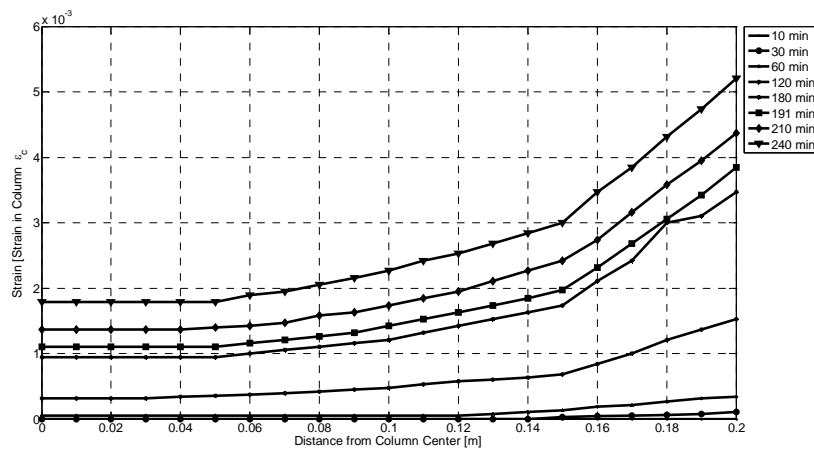
Figure 7: Variation of Strain in Column for Case 1 along Path 1
