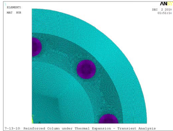
Figure 4: Finite Element Mesh of RVE
