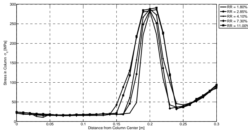
Figure 11: Variation of Stress in Column with Different Reinforcing Ratio
