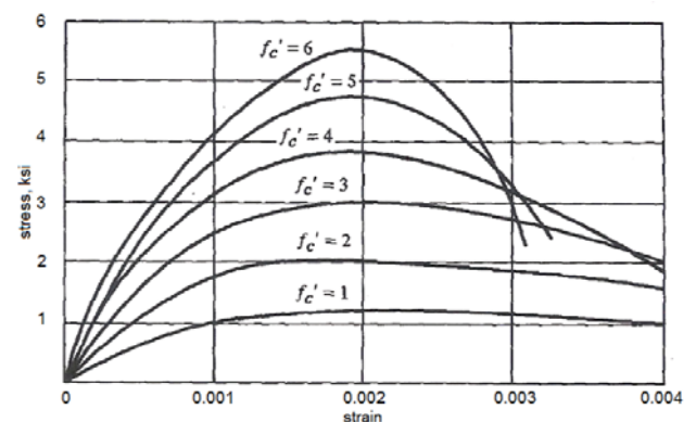
Figure 1: Typical Concrete Stress-Strain Curves (1 ksi = 6895 kPa), (McCormac 2008)
