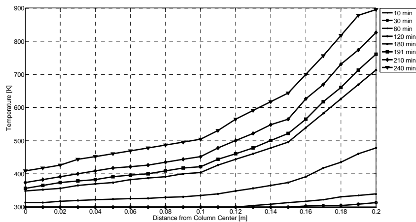
Figure 6: Temperature Distribution for Case 1 along Path 1
