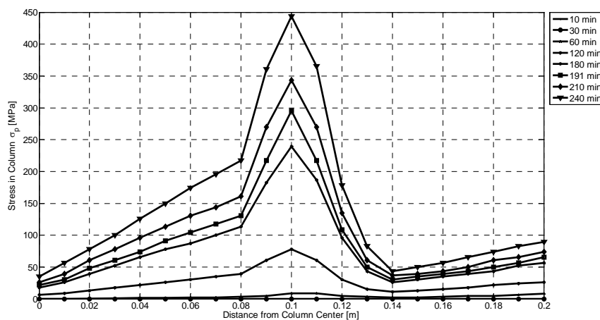
Figure 9: Variation of Stress in Column for Case 1 along Path 2
