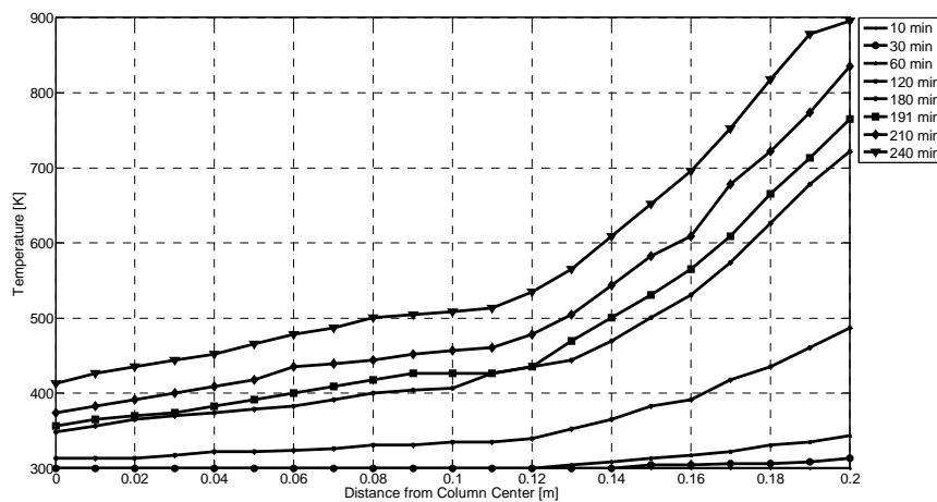
Figure 8: Temperature Distribution for Case 1 along Path 2
