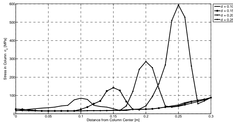
Figure 10: Variation of Stress in Column with Varying Rebar Array Radius ( t = 180\text{min} )
